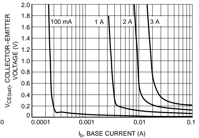
Figure 15. Saturation Region
