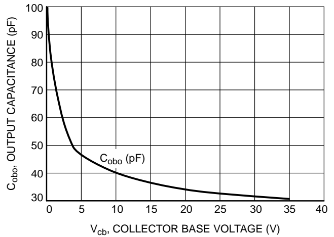
Figure 17. Output Capacitance
